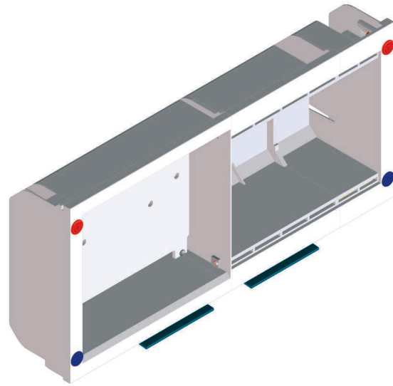
Size 2: ER end housing (left) for mounting the controller with various mounting rails, ER middle housing and ER end housing (right) for mounting 19" modules with a width of up to 33 HP
